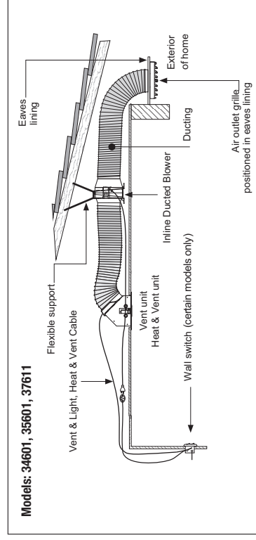
Fig. 2: Layout of Tastic Luminate® Vent, Vent & Light, and Heat & Vent Modules.
