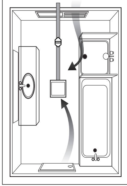
Fig. 1: Ideal placement of Tastic®. Sufficient air inlets into room are required
